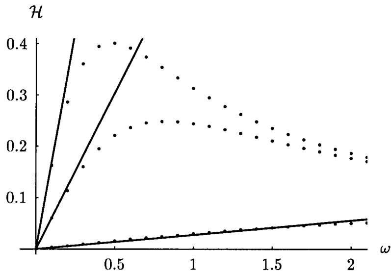
Figure 6. Hysteresis \mathcal{H} versus \omega illustrating the low-frequency expansion of the hysteresis. Straight lines: Expression (18) evaluated numerically. Top: Low temperature ( \tau = 0.5 ). Middle: Moderate temperature ( \tau = 1 ). Bottom: High temperature ( \tau = 10 ).
