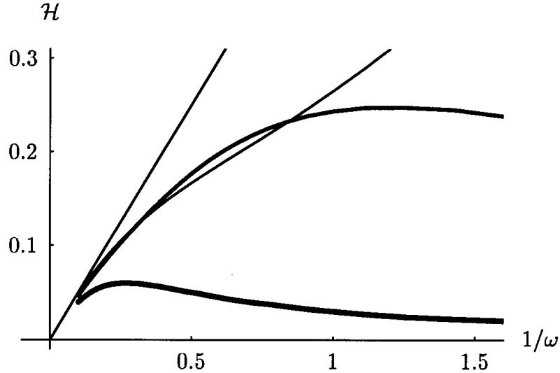
Figure 5. Hysteresis \mathcal{H} versus 1/\omega illustrating the high-frequency expansion of the hysteresis. Straight line: Expression (14), i.e., \mathcal{H} \sim \alpha / \omega = 1/2/\omega Thin line: Low temperature ( \tau = 0.1 ). Medium line: Moderate temperature ( \tau = 1 ). Thick line: High temperature ( \tau = 10 ).
