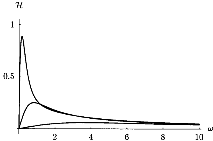
Figure 4. Hysteresis \mathcal{H} , as defined in (10), versus frequency \omega for several temperatures. Top: Low temperature ( \tau = 0.1 ). Middle: Moderate temperature ( \tau = 1 ). Bottom: High temperature ( \tau = 10 ).
