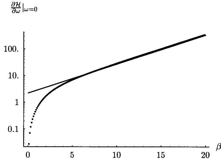
Figure 7. \frac{\partial \mathcal{H}}{\partial \omega}|_{\omega=0} versus \beta showing low-temperature (large- \beta ) agreement. Dotted line: Evaluation according to the low-frequency expansion. Straight, solid line: Evaluation according to (23).
