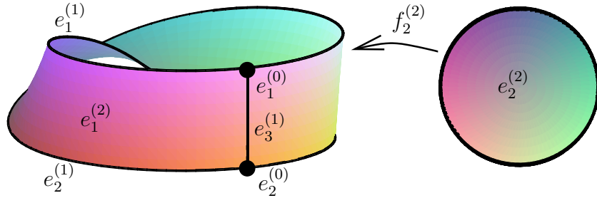
Figure 5.1: A CW complex for \mathbb{RP}^2
