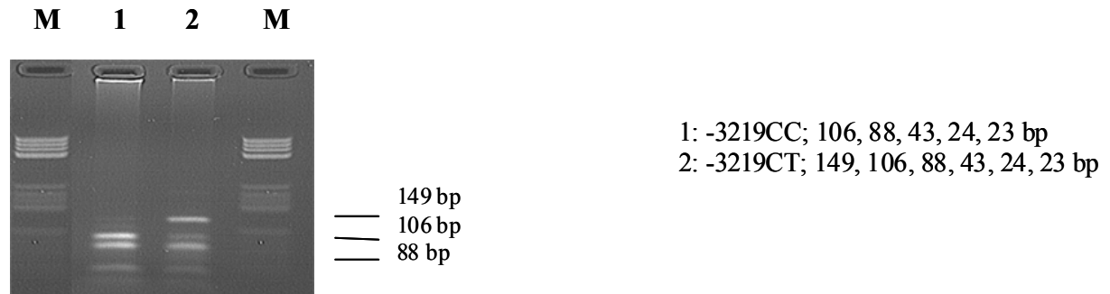
Abb. 10: BsII digest of a 284-bp fragment containing the positions of the m6 mutation.
