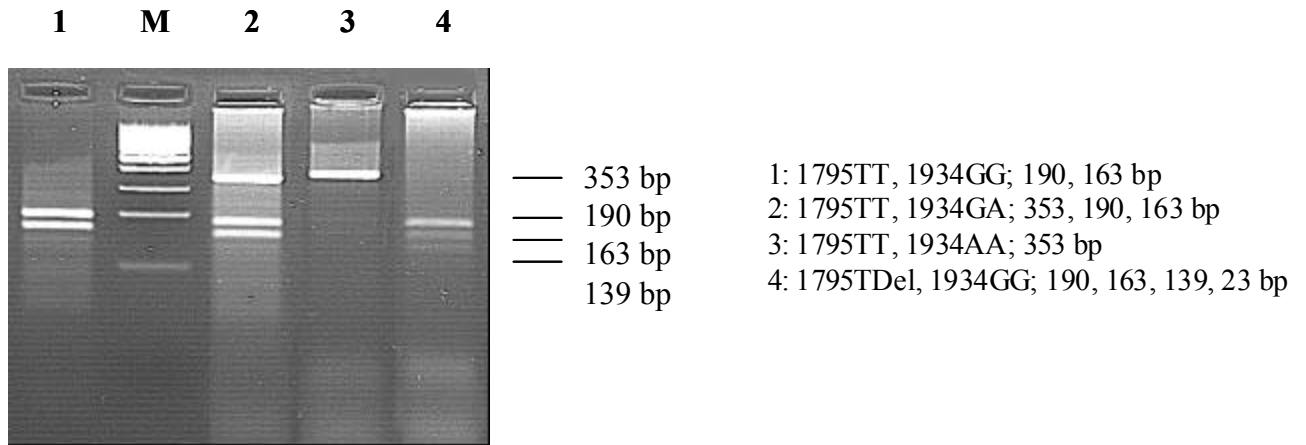
Figure 13: Bst NI digest of a 353-bp fragment containing the mutations 1795T>Del and 1934G>A of the CYP2D6 gene.
