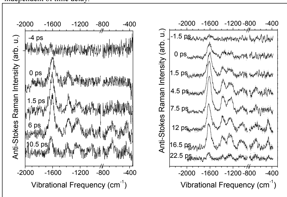
Fig.5.13: Transient anti-Stokes Raman spectra of B-30 dissolved in PC (left) and GTA (right).
