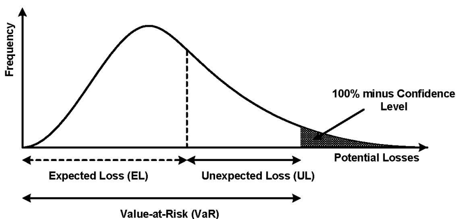
Figure 1: Loss distribution
