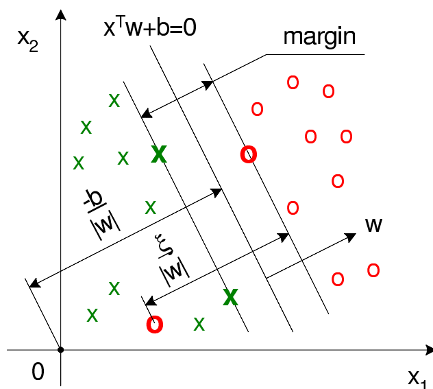
Figure 2: Separating hyperplane
