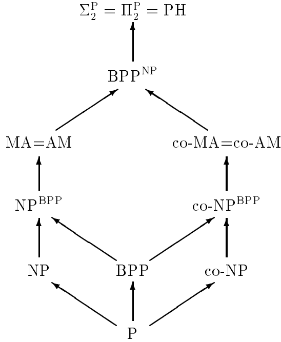
Figure 2: The classes under the assumption NP \subseteq P/poly .
