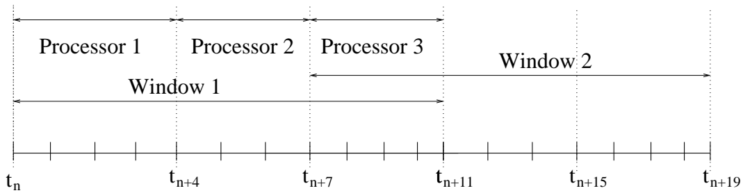
Figure 1: Parallelization of the time intervals.
