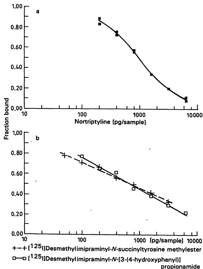
Fig. 3. Standard curve for a) nortriptyline and b) [ ^{125} I]desmethylimipraminyl-N-succinyltyrosine methylester (---) and [ ^{125} I]desmethylimipraminyl-N-[3-(4-hydroxyphenyl)]propionamide (—□—). The measurements were carried out in triplicate.
