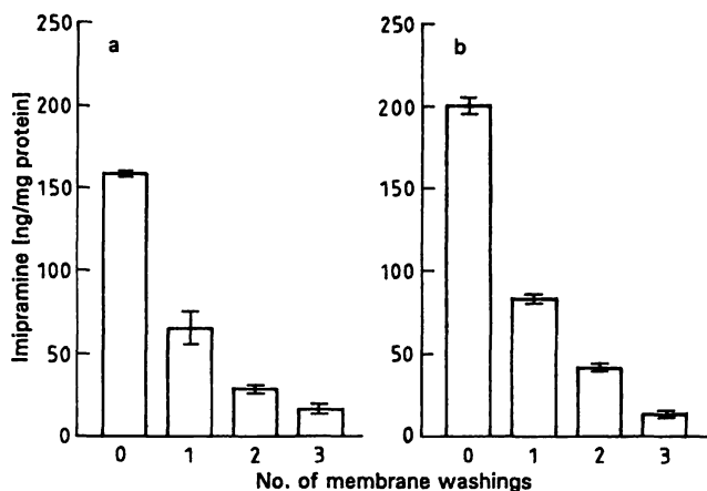
Fig. 5. Rate of dissociation of imipramine bound to erythrocyte membranes. The determination was carried out using a) [ 3 H]imipramine and b) RIA with the same concentration of bound imipramine. Erythrocyte membranes were incubated with imipramine hydrochloride (1 µmol/l) in ice-cold buffered solution (50 mmol/l Tris, 120 mmol/l NaCl, 5 mmol/l KCl, pH 7.4) for 60 min. The membranes were repeatedly washed and centrifuged (40000 g, 10 min). Imipramine was extracted (see Methods) and determined by RIA. The same method was used with addition of 3 nmol/l [ 3 H]imipramine and radioactivity was measured.
