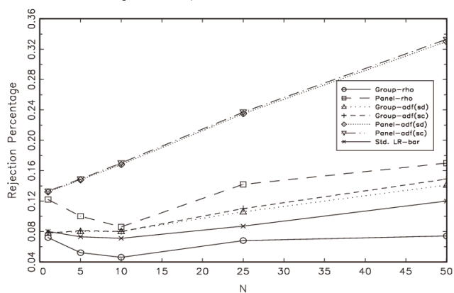
Figure 4: Empirical Size Results for T=100
