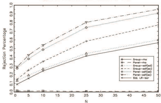
Figure 2: Empirical Size Results for T=25
