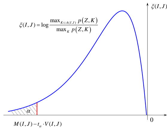
Figure 3.3: Calculation of critical value t_\alpha
