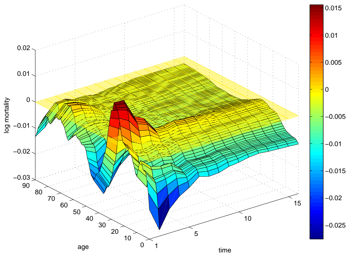
Figure 3: Surface of the median response of logarithmized age-specific male mortality to a one standard deviation shock in unemployment in the U.S. 1956–2004. The time axis refers to the time elapsed since the impulse and the yellow grid marks the zero plane.
