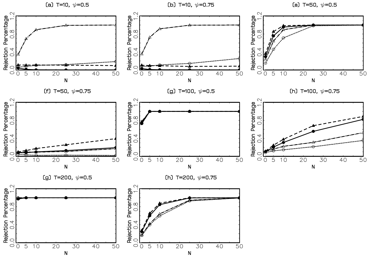
Figure 5: Empirical power results of the tests for DGP B and true cointegrating rank of two when hypothesized rank is one. ●—— panel SL-asympt, ▲ — — — panel SL-VAR(1), ○..... LLL-asympt, △ - · - · - LLL-VAR(1).
