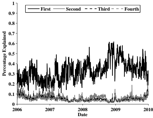
5.1: Blocked Kernel
