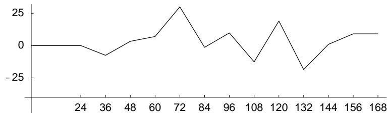
FIG. 9. Difference of mean values of the reduced and initial scenario trees
