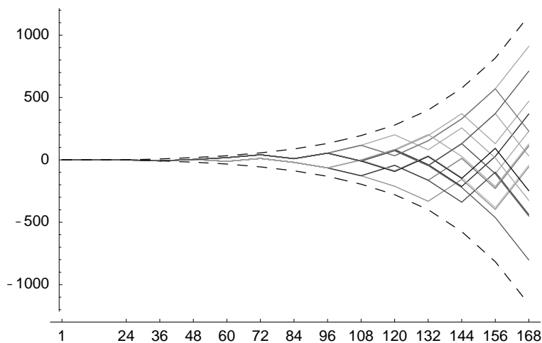
FIG. 8. Shifted supports of the reduced scenario tree
