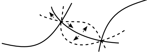
Figure 2.20: How the general fiber of a family in (S18) moves
