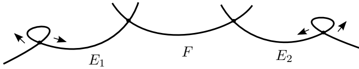
Figure 2.9: How the general fiber of a family in (S7) moves
