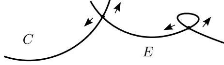
Figure 2.5: How the general fiber of a family in (S3) moves
