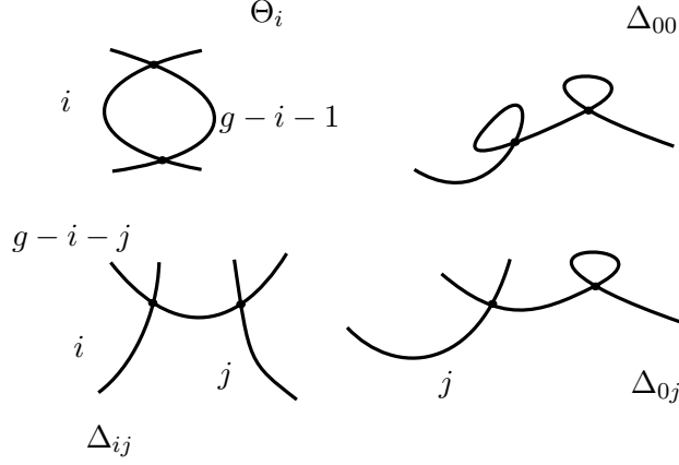
Figure 2.1: Loci in \overline{\mathcal{M}}_g
