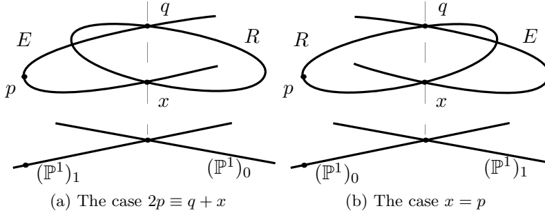
Figure 2.2: The admissible covers for the two fibers of the family \overline{C} when g = 2
