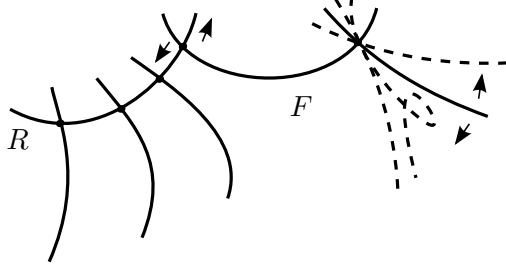
Figure 2.13: How the general fiber of a family in (S11) moves
