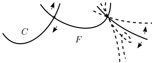
Figure 2.8: How the general fiber of a family in (S6) moves
