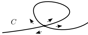
Figure 2.17: How the general fiber of a family in (S15) moves
