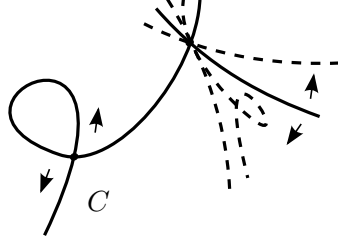
Figure 2.16: How the general fiber of a family in (S14) moves
