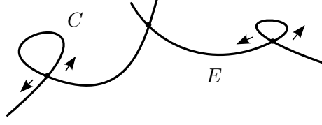
Figure 2.15: How the general fiber of a family in (S13) moves
