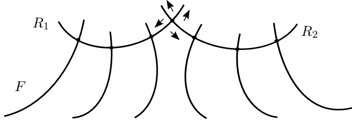
Figure 2.12: How the general fiber of a family in (S10) moves
