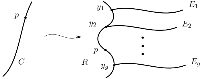
Figure 1.2: Degeneration of a general pointed curve
