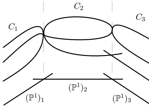
Figure 1.1: An admissible cover
