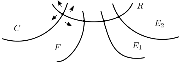
Figure 2.11: How the general fiber of a family in (S9) moves
