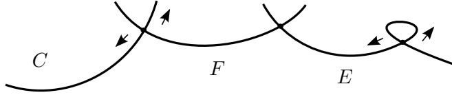
Figure 2.6: How the general fiber of a family in (S4) moves
