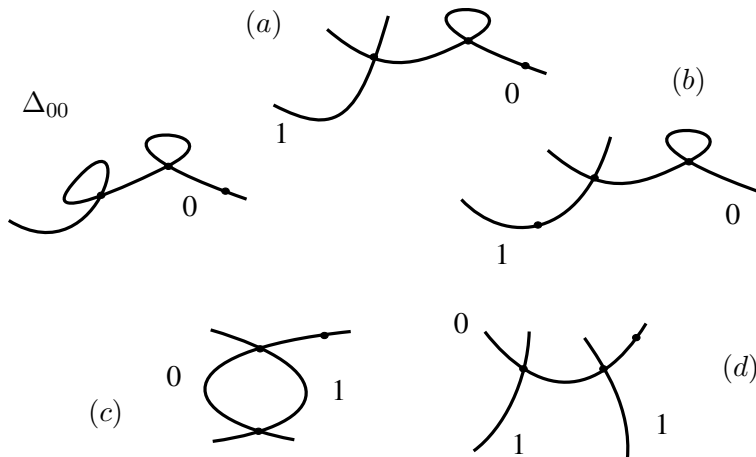
Figure 2.21: Loci in \overline{\mathcal{M}}_{2,1}
