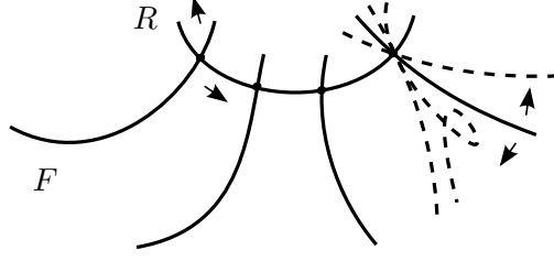
Figure 2.14: How the general fiber of a family in (S12) moves
