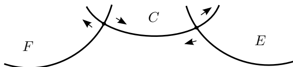
Figure 2.18: How the general fiber of a family in (S16) moves
