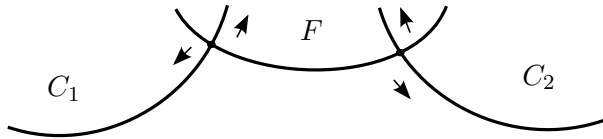
Figure 2.4: How the general fiber of a family in (S2) moves
