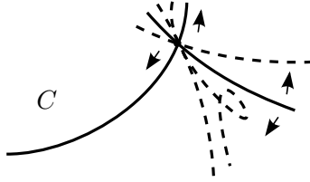
Figure 2.7: How the general fiber of a family in (S5) moves
