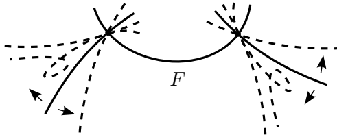
Figure 2.10: How the general fiber of a family in (S8) moves
