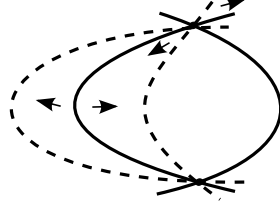
Figure 2.19: How the general fiber of a family in (S17) moves
