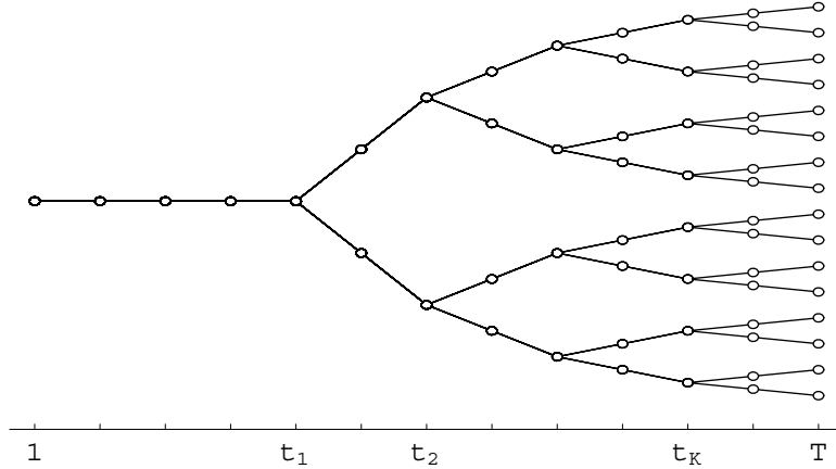
Fig. 1. Example of a (binary) scenario tree
