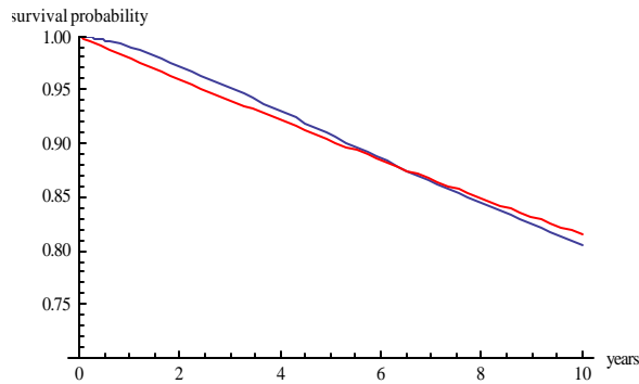
Figure 6: Survival probabilities implied by the Nelson Siegel fitting procedure (blue curve) and CIR model with fitted parameters \mathbf{a} , \mathbf{s} and \mathbf{q} for 25.03.2008
