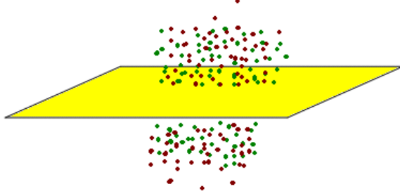
Figure B.2: Non-Gaussian component analysis for the classification problem. We assume that the useful signal for both populations belongs to the same low-dimensional subspace \mathcal{S} ; rest parts have normal distribution, but with different covariance matrices.
