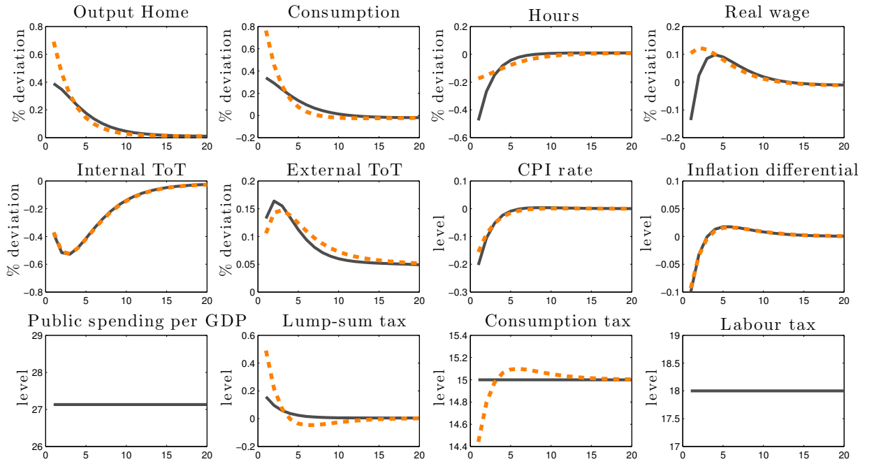
Figure 2: Impulse response functions after a shock to Z_N of one standard deviation. baseline = solid line, responsive rule (1) = orange dotted line.
